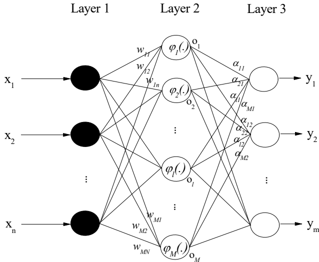
Fig. 4 Single-hidden layer neural network
