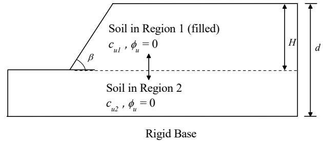
Fig. 2 Problem configuration for cohesive material filled on purely cohesive soil
