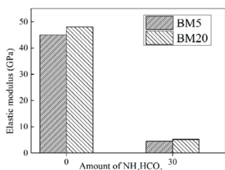
Fig. 7 Elastic modulus of sintered solid and porous Ti-20Nb-5Ag of BM5 and BM20
