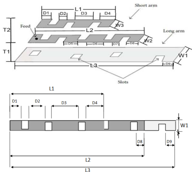
Fig. 2 Geometry of the wideband antenna
