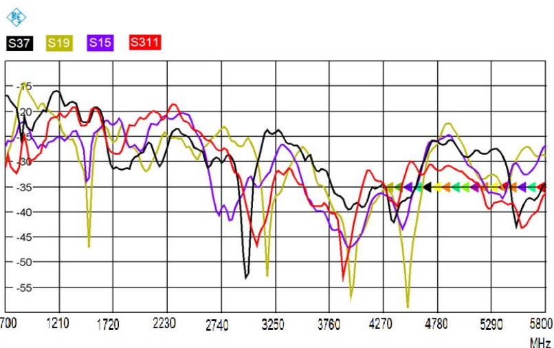
Fig. 13 The lowest isolation between the 12 MIMO antennas mounted on small size mobile handset
