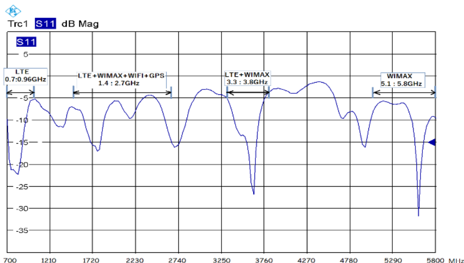
Fig. 3 Measured return loss of the antenna
