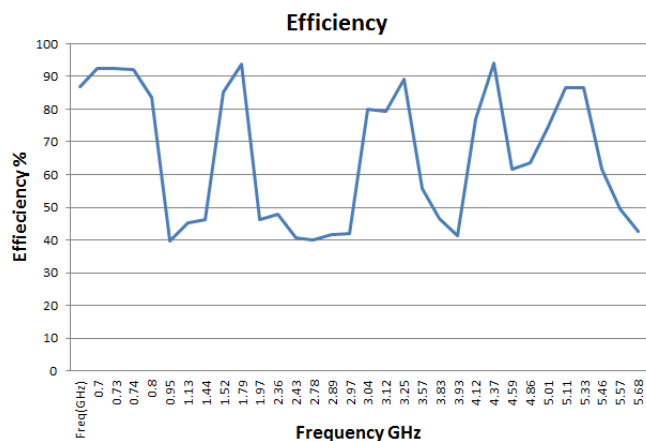
Fig. 4 Measured efficiency of the antenna
