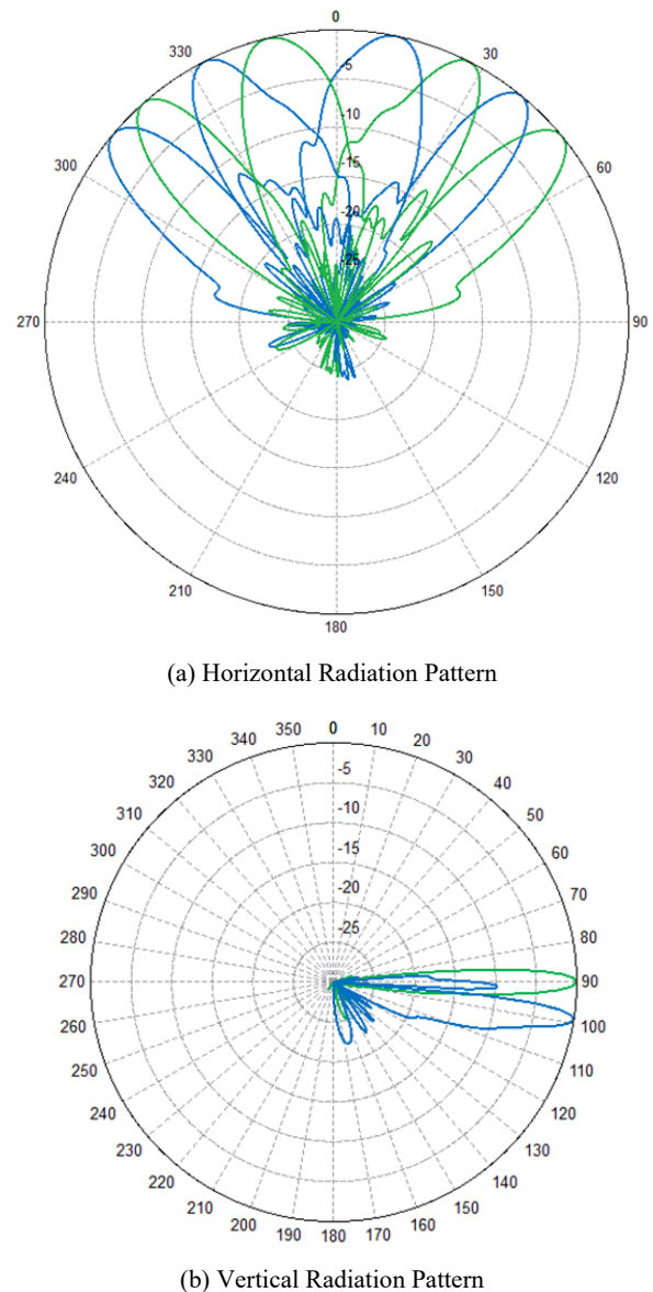
Fig. 10 Peaks of one vertical group of beams aligned above (or close to) nulls of the other group at 1.8 GHz
