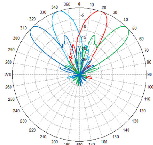
(a) Horizontal Radiation Pattern
