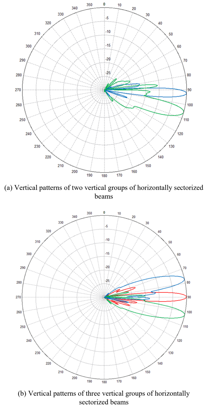
Fig. 9 Different configurations of vertical sectorization at 1.8 GHz
