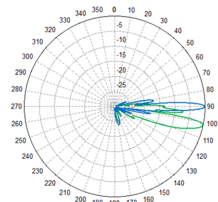
(b) Vertical Radiation Pattern
