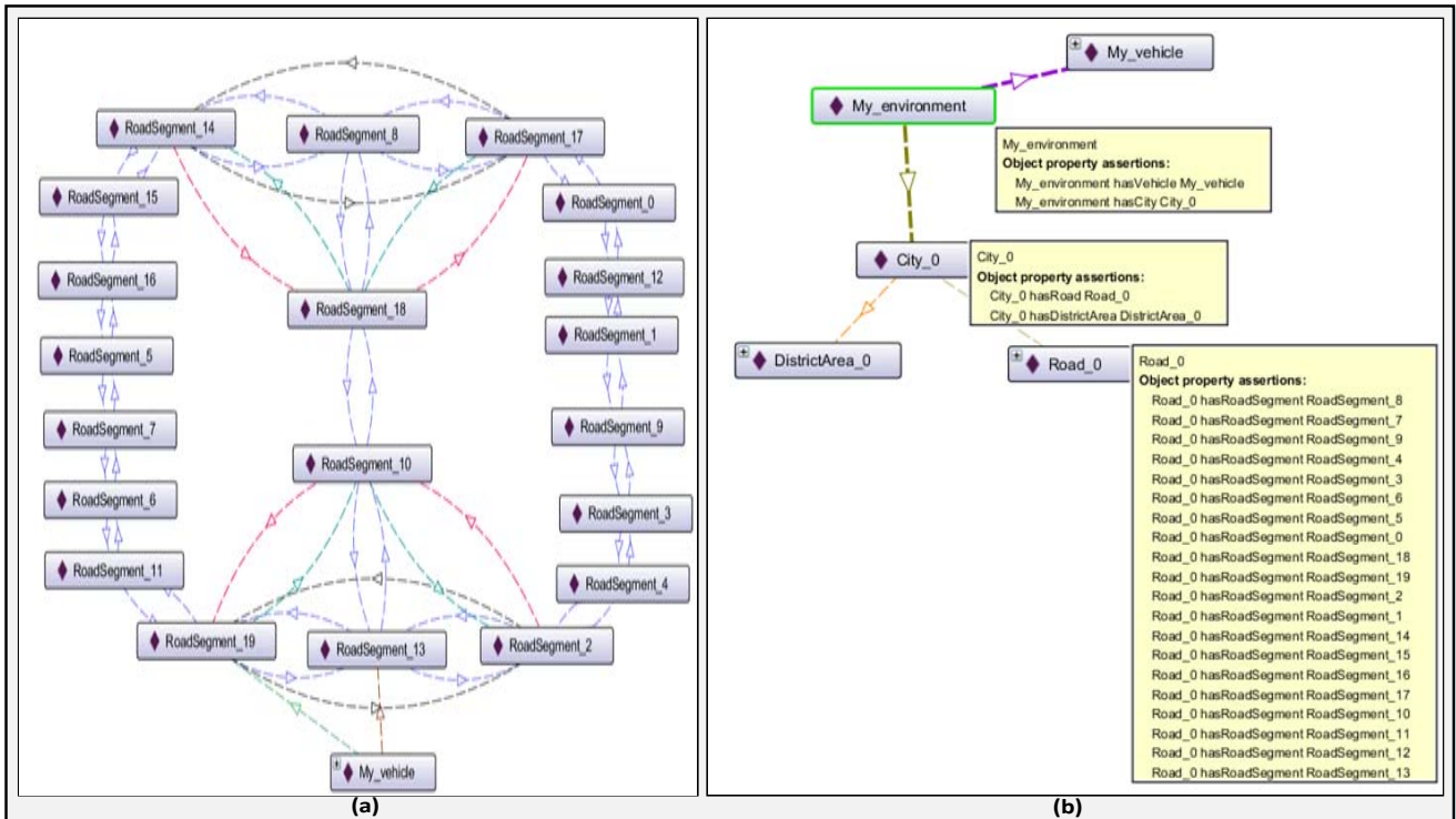
Fig. 11 (a) The ontological representation of road segments. (b) The individuals of various classes (vehicle, and individuals for various environment classes) for the simulated turn right driving event
