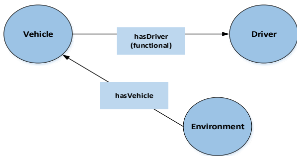
Fig. 2 Ontology for the driving context
