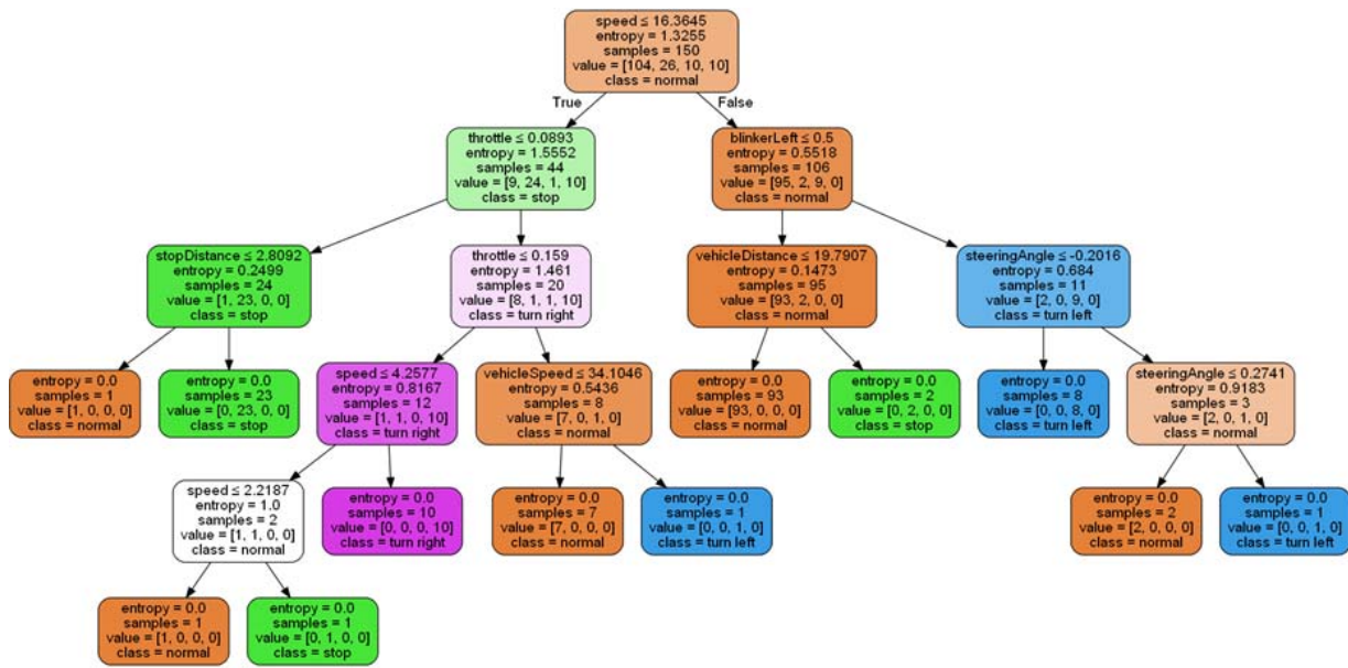
Fig. 12 Classification tree example
