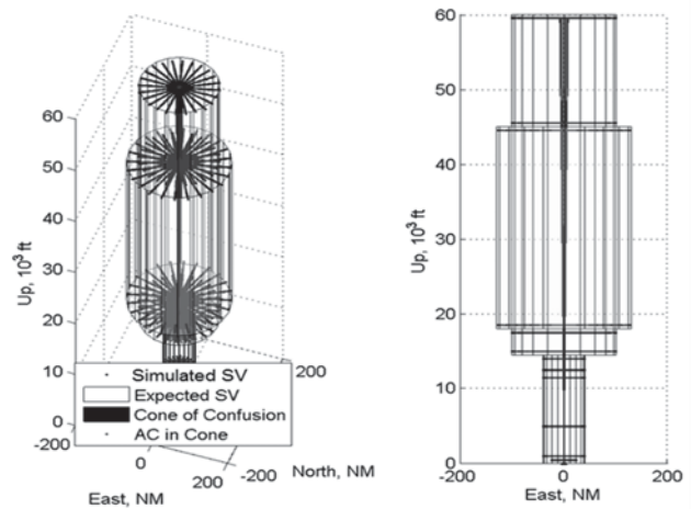
Fig. 6 High-altitude VOR (HVOR) Service Volume (SV)
