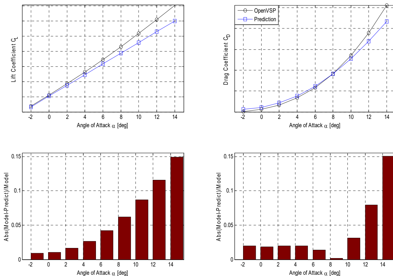
Fig. 8 Lift and drag coefficient comparison for Mach number equal to 0.9
