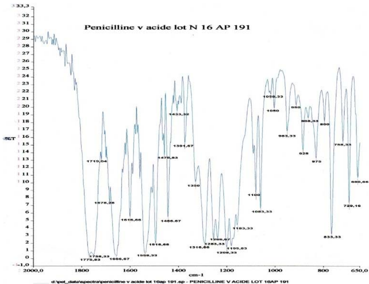
Fig. 3 Penicillin V acid Infrared Spectra
