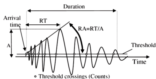
Fig. 1 The typical AE signal features [11]
