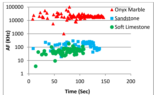
Fig. 5 Variation of average frequency with time for the three rock types
