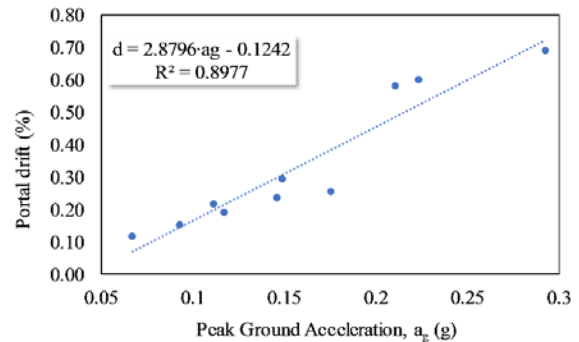
Fig. 7 Portal drift vs PGA
