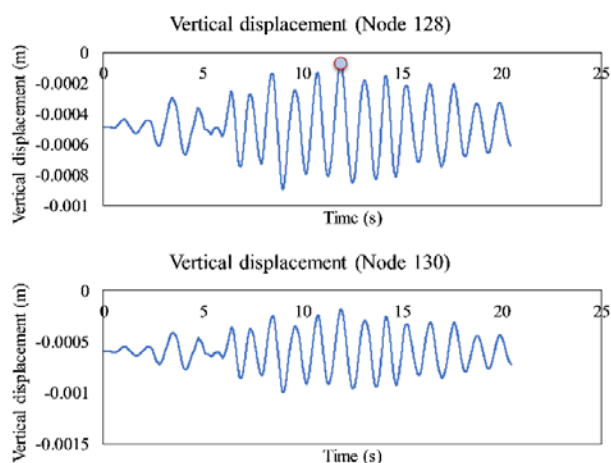
Fig. 8 Vertical displacement of landside legs under artificial ground motion ZISE
