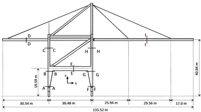
Fig. 2 Overview of Jumbo container crane
