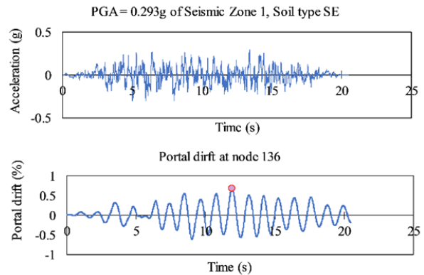
Fig. 6 Portal drift on node 136 under seismic Z1SE
