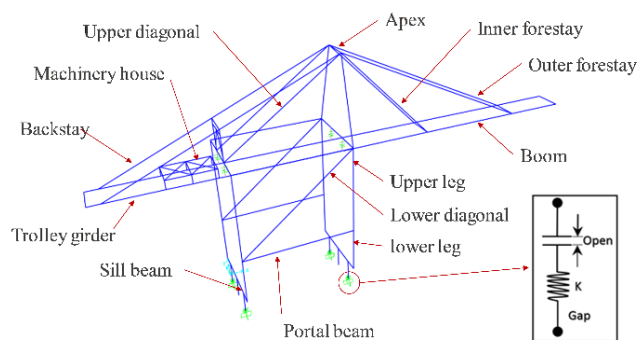
Fig. 1 3D model of jumbo container crane
