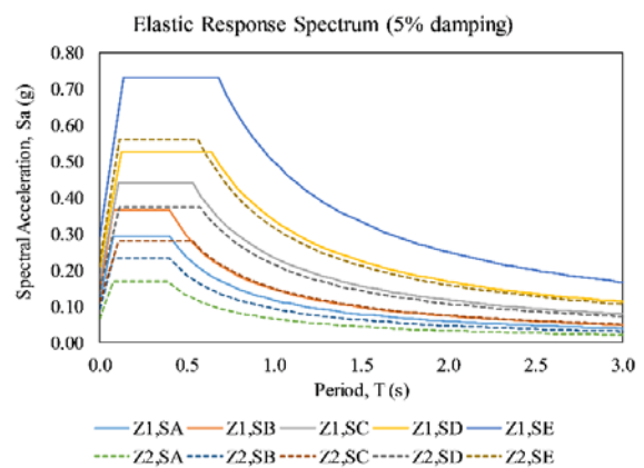
Fig. 4 Elastic response spectrum developed from KBC 2005
