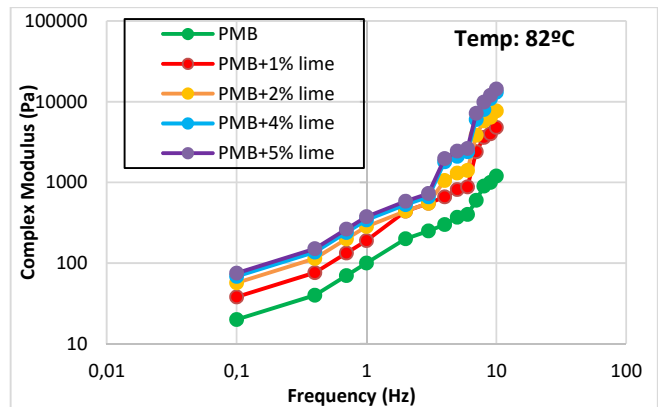
Fig. 4 Effect of lime on complex modulus at 82 °C
