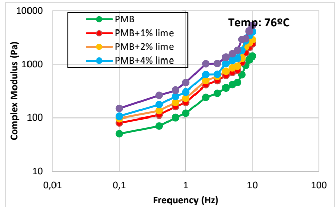
Fig. 3 Effect of lime on complex modulus at 76 °C
