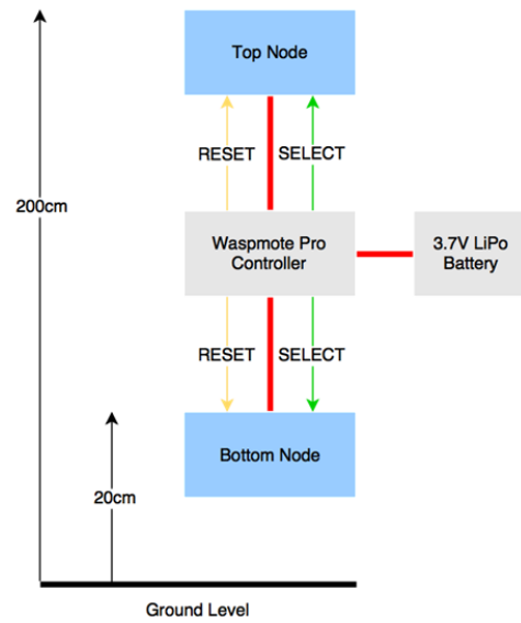
Fig. 4 Block diagram of range test apparatus
