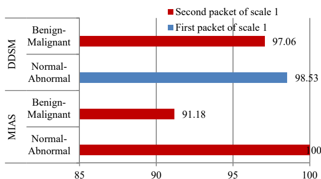
Fig. 3 The accuracy results for the packets which provide the best classification performance
