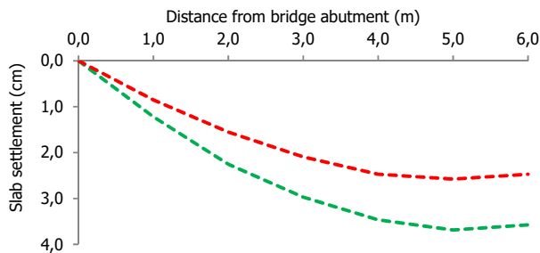
Fig. 5 Settlements calculate analytically, Green line shows the settlement when soil subgrade reaction is taken 24.000 kN/m 3 , Red line shows the settlement when soil subgrade reaction is taken 32.000 kN/m 3
