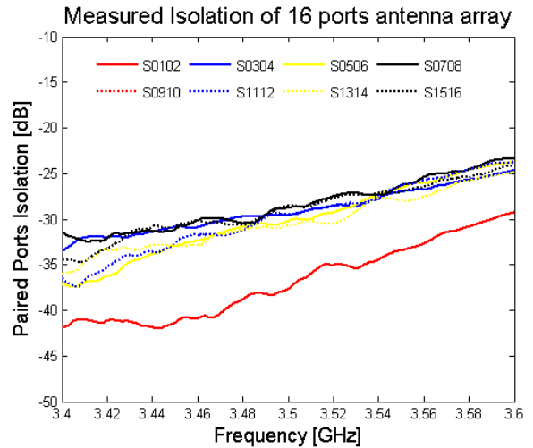
Fig. 5 Measured isolation of 16 ports antenna array
