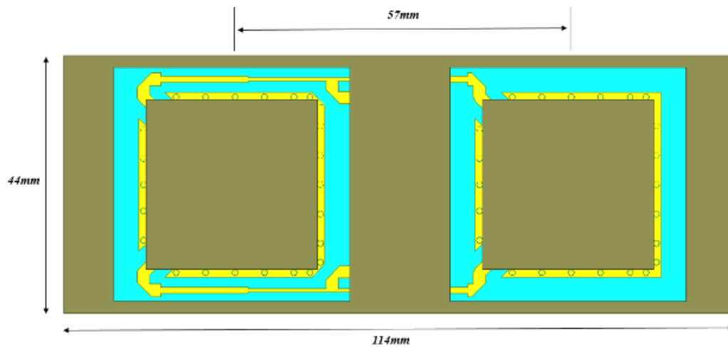
Fig. 2 Top View of the 2 x 1 antenna element
