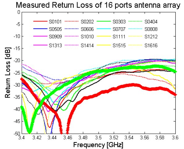
Fig. 4 Measured return loss of 16 ports antenna array
