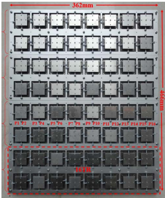
Fig. 3 Fabricated 64 RF ports antenna array
