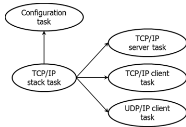
Fig. 4 Application threads
