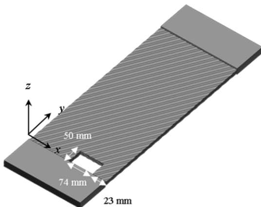
Fig. 1 Geometry of heating element and plugging
