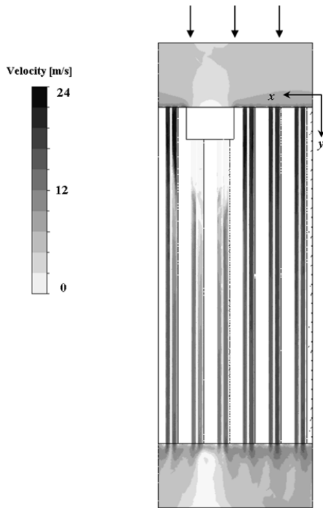
Fig. 3 Velocity distribution of heating element with plugging
