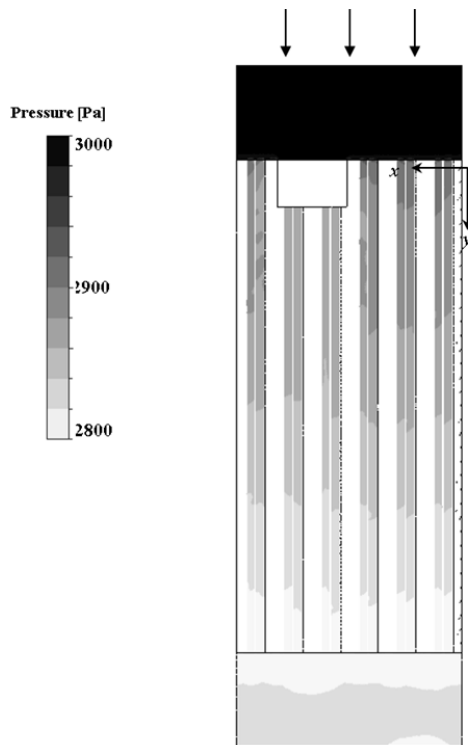
Fig. 4 Pressure distribution of heating element with plugging
