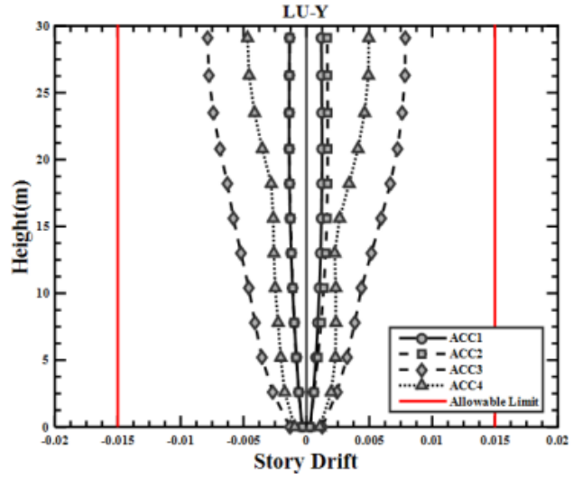
(c) Story drift in LU on Y-axis
