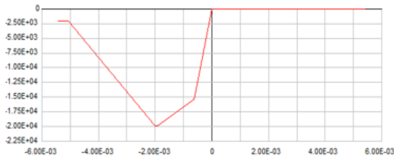
(a) Concrete model (Mander model)
