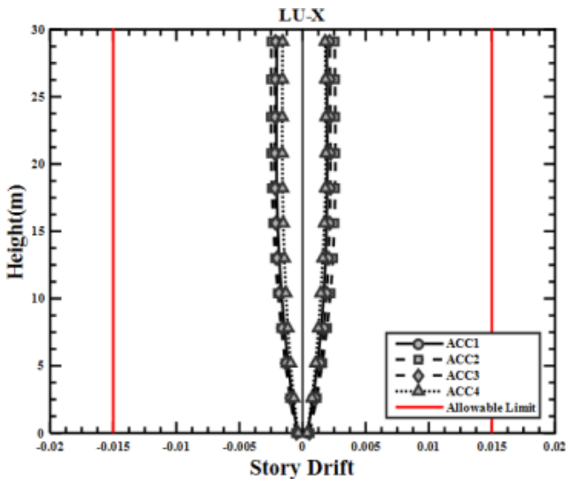
(b) Story drift in LU on X-axis
