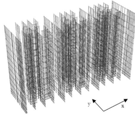
Fig. 1 Shear wall building model (Perform-3D)
