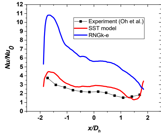
Fig. 2 Validation of local heat transfer distribution
