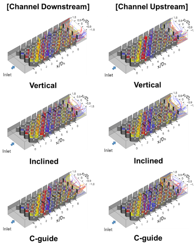
Fig. 4 Streamline of various rib configurations channels
