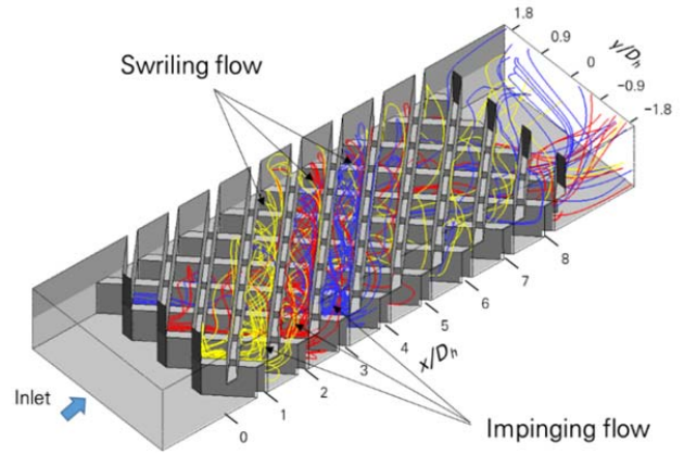
Fig. 3 Streamline of base case
