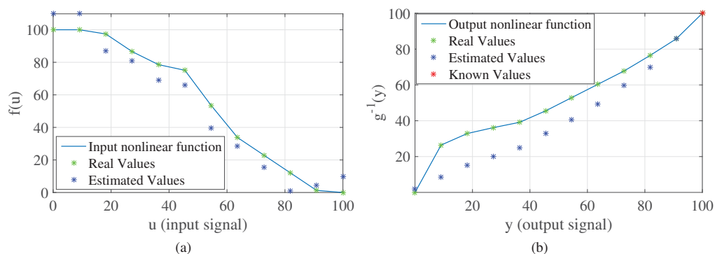
Fig. 6 Estimating input and output functions in instant H-W system by using constrained linear least-squares algorithm, after quantization input of f and g^{-1} to 12 parts in u and y axes and considering only one known point
