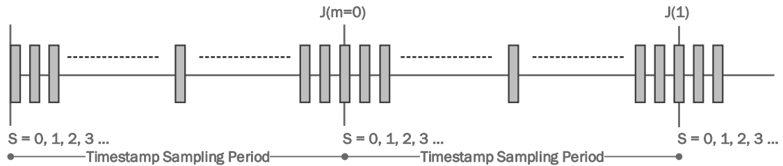
Fig. 2 Clock synchronization algorithm – sampling periods
