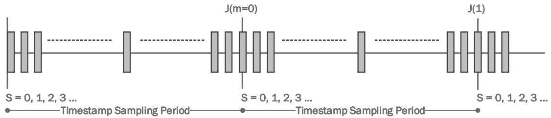
Fig. 2 Clock synchronization algorithm – sampling periods
