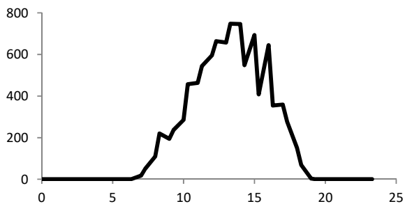
Fig. 2 Solar Radiation ( \text{Js}^{-1}\text{m}^{-2} ) against Time Intervals (GMT)
