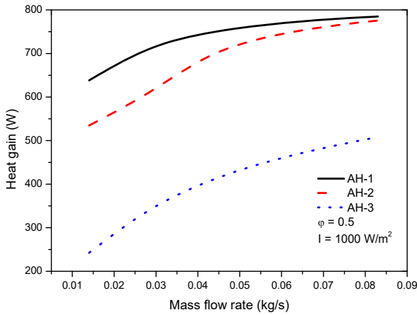
Fig. 3 Heat gain vs. mass flow rate
