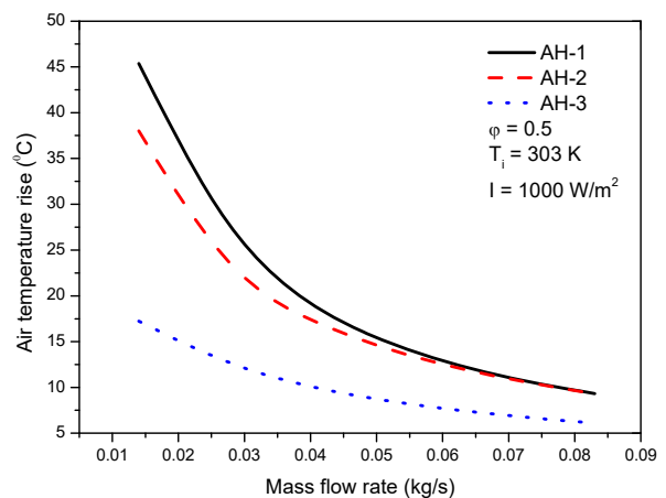
Fig. 2 Air temperature rise vs. mass flow rate
