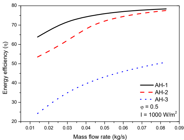
Fig. 4 Energy efficiency vs. mass flow rate
