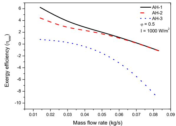
Fig. 6 Exergy efficiency vs. mass flow rate
