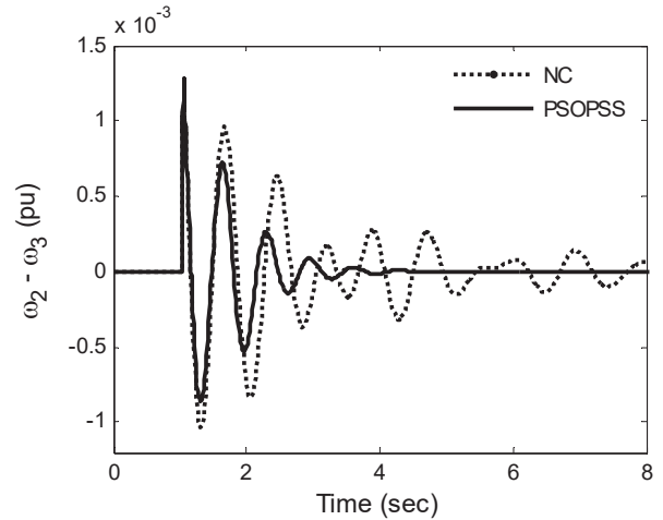
Fig. 12 Local mode of oscillation for self clearing 3-phase fault near bus5
