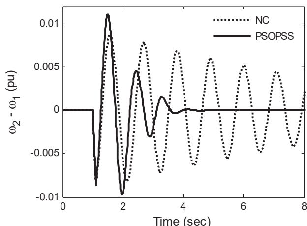
Fig. 14 Inter-area mode of oscillation under small disturbance
