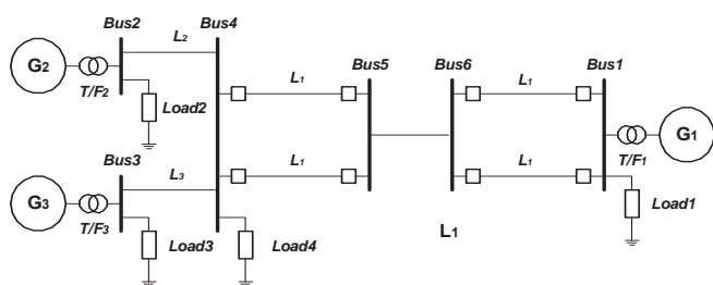
Fig. 1 Multi-machine power system
