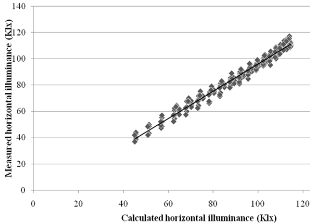
Fig. 4 Comparison of the measured and calculated mean values on horizontal illuminance
