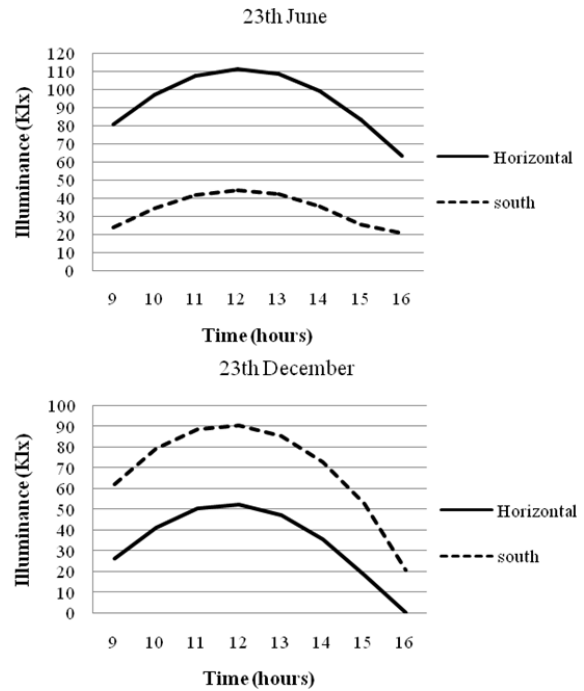
Fig. 5 Global horizontal and south facing vertical illuminance values for two clear days in summer (23 rd June) and winter (23 rd December) in Tehran, Iran
