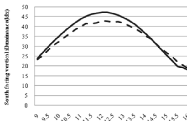
Fig. 2 Comparison of the measured and calculated mean values on the south facing vertical. --- Measured Vertical Illuminance, — Calculated Vertical Illuminance
