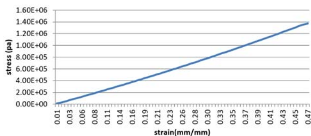
Fig. 12 Stress-strain diagram based on the proposed model
