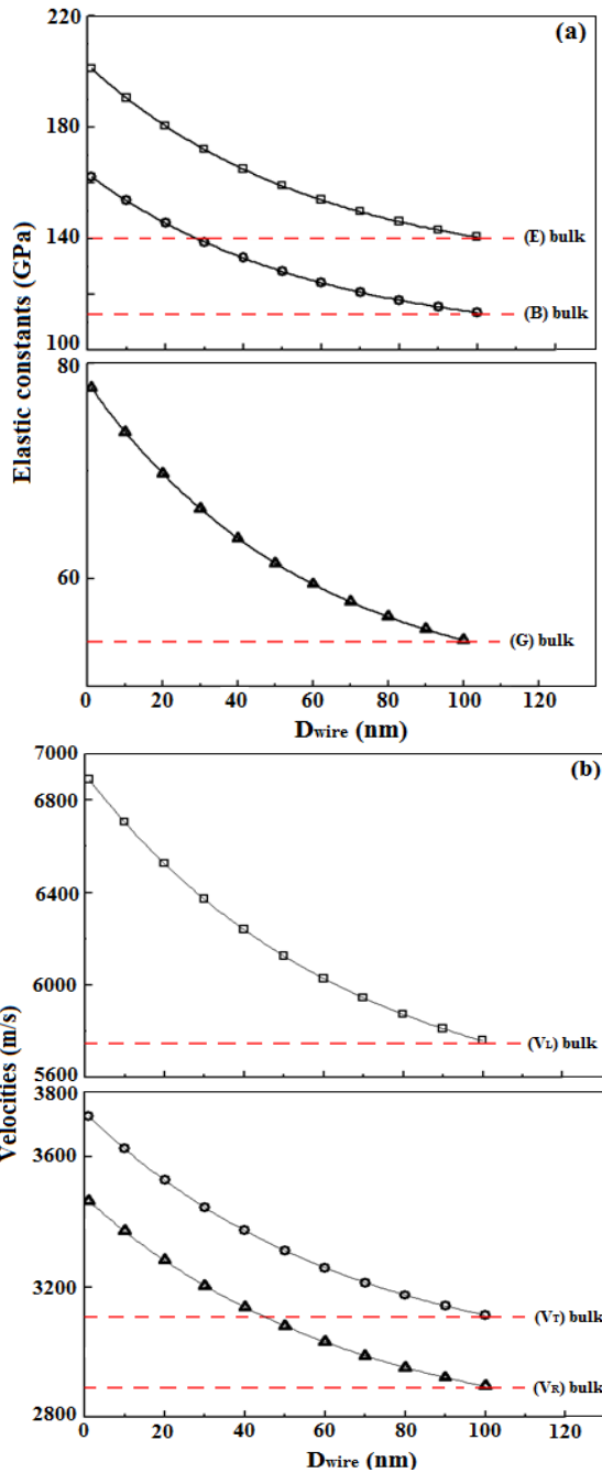
Fig. 3 Effects of ZnO wire diameters ( D_{\text{wire}} ) on (a) elastic constants: E (□), B (○) and G (Δ) and (b) velocities: V_L (□), V_T (○) and V_R (Δ). The horizontal dashed lines represent the corresponding calculated bulk value along the [0001] direction
