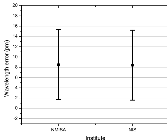
Fig. 3 Wavelength scale calibration comparison between NIS and NMISA for wavelength range 1530-1560 nm
