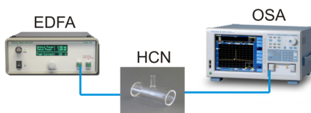
Fig. 2 OSA calibration setup using H13CN reference gas cell
