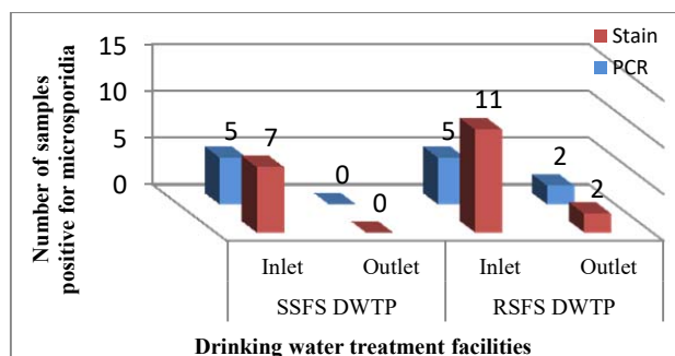
Fig. 2 Comparison between light microscopy and PCR for the detection of Microsporidial spores
