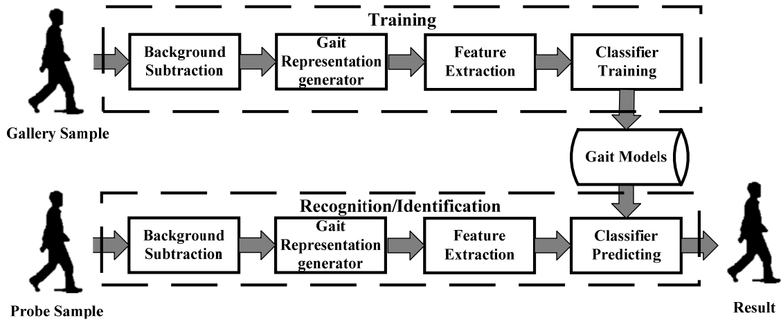
Fig. 1 Gait recognition system overview
