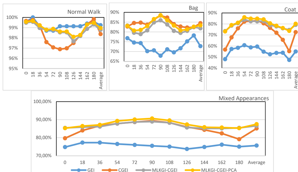
Fig. 6 CCR in each appearance
