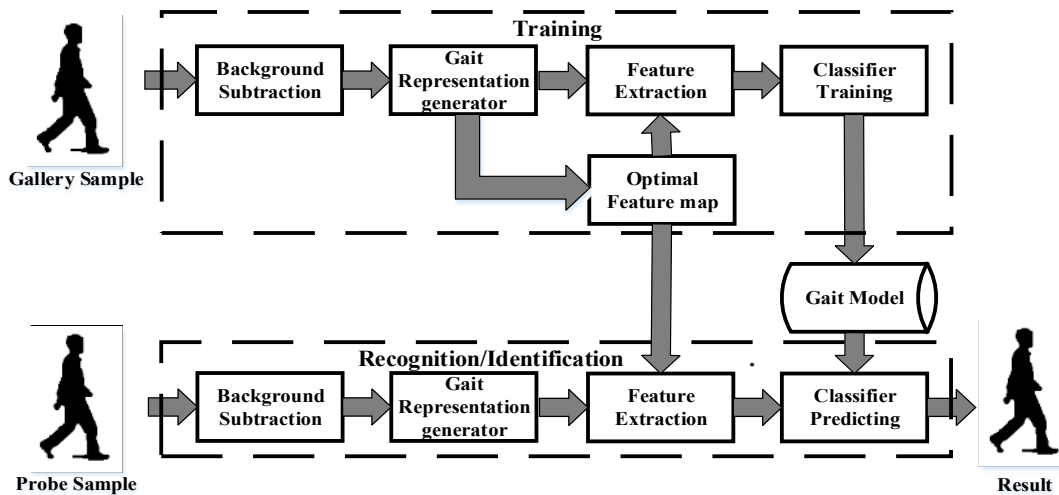
Fig. 5 Gait recognition system
