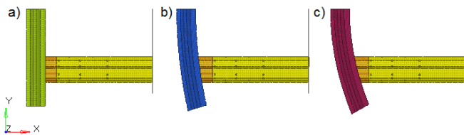
Fig. 4 Beam curvature cases: (a) straight, (b) medium radius, (c) maximum radius
