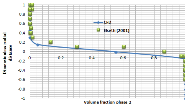
Fig. 4 Comparison of water volume fraction profile with Elseth [3]
