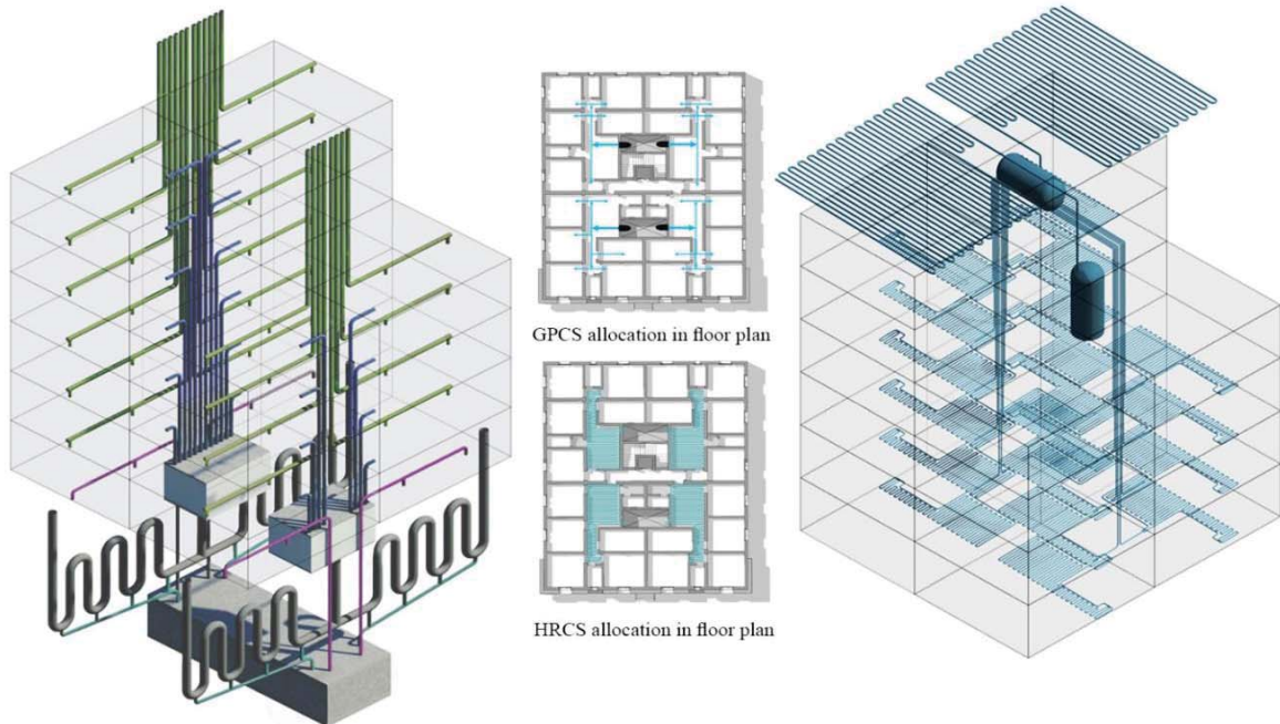
Ground Pipe Cooling System (GPCS) Model
