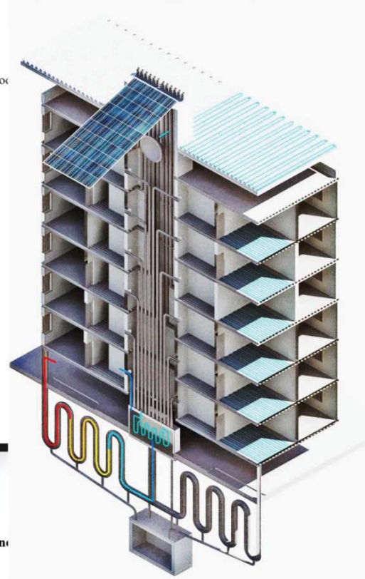
Hydronic Radiant Cooling System (HRCS) Model
