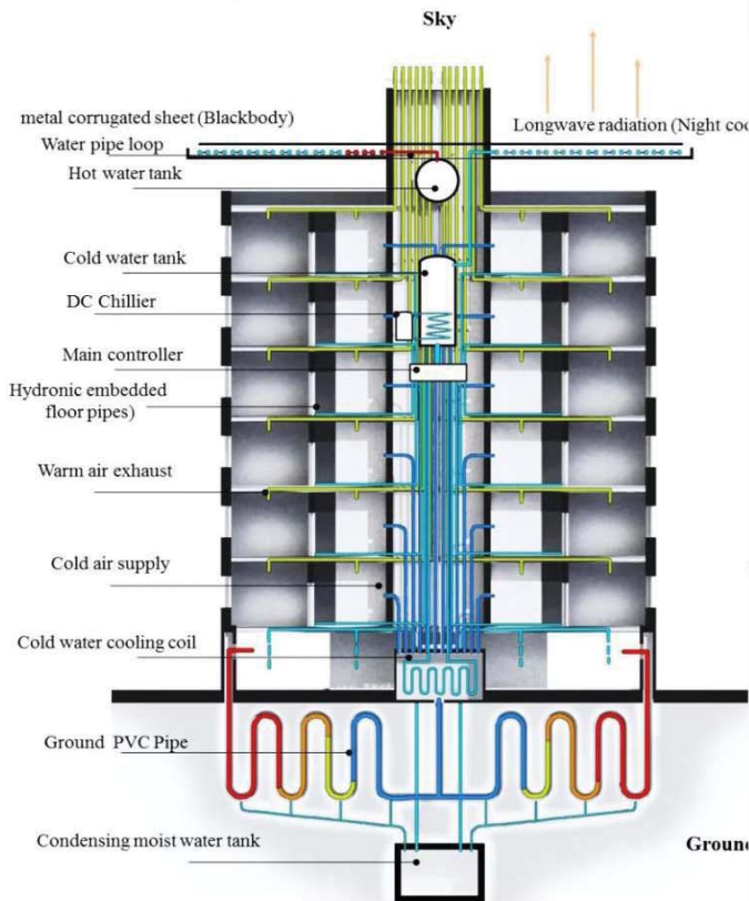
Ground Pipe Cooling System (GPCS) Model
