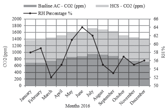
Fig. 9 Comparative assessment of HCS indoor air quality
