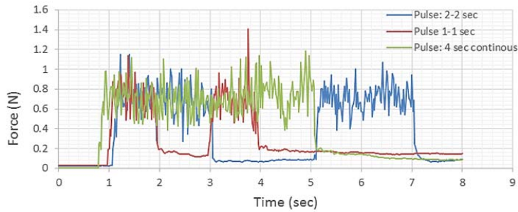
Fig. 7 Bubble collapse force (N) at different pulse on-off timing in seconds at 108μm amplitude
