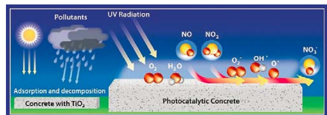
Fig. 1 Photocatalytic principle
