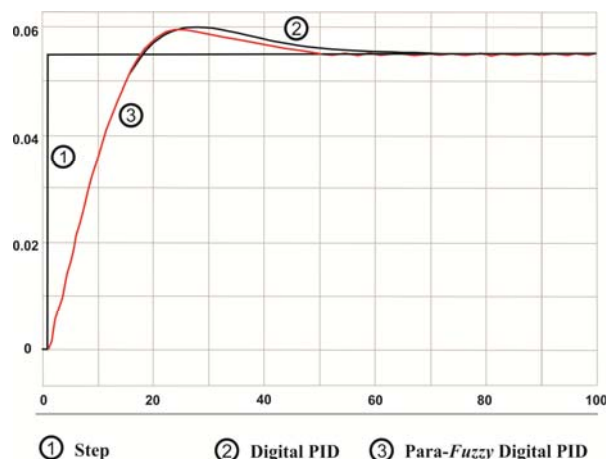
Fig. 14 Comparison of the Para-Fuzzy Digital PID with conventional Digital PID in response to 0.055 m step. (1) 0.055 m step; (2) Response of conventional Digital PID; (3) Response of Para-Fuzzy Digital PID
