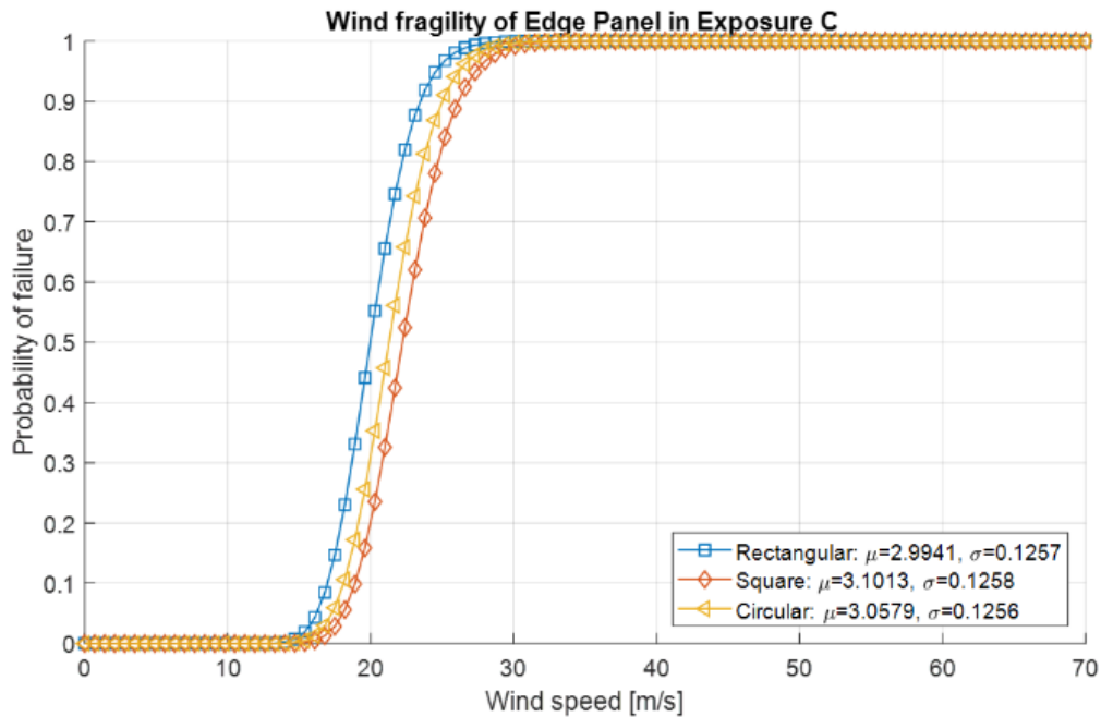
Fig. 10 Edge soundproof wall fragility curves for section shape (exposure C)
