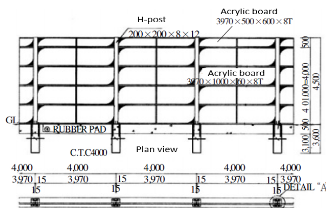
Fig. 2 Shape and specification of sound proof structure
