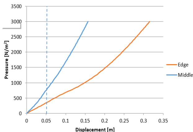
Fig. 6 Resistance capacity for edge and middle soundproof wall
