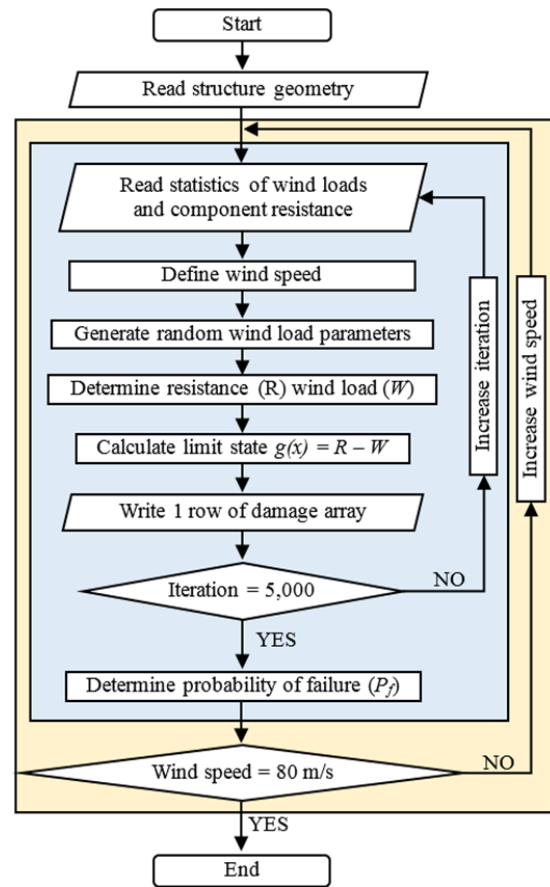
Fig. 7 Monte Carlo Simulation flowchart
