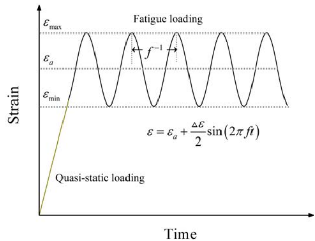
Fig. 4 Loading profile of HTPB propellant
