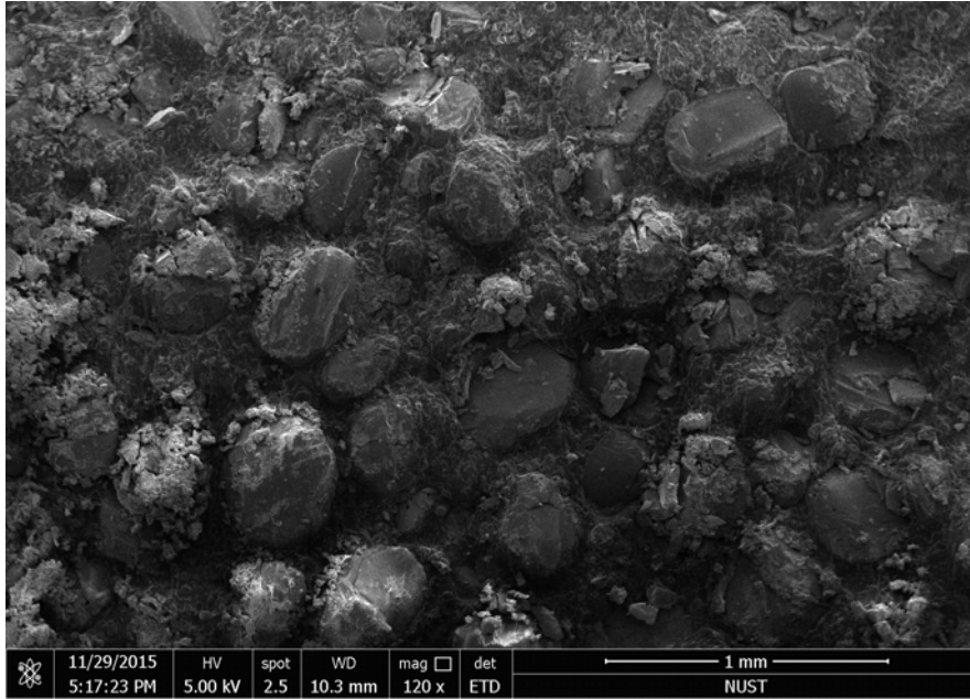
Fig. 1 SEM image of HTPB propellant
