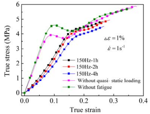
(a) Identical frequency with various fatigue time
