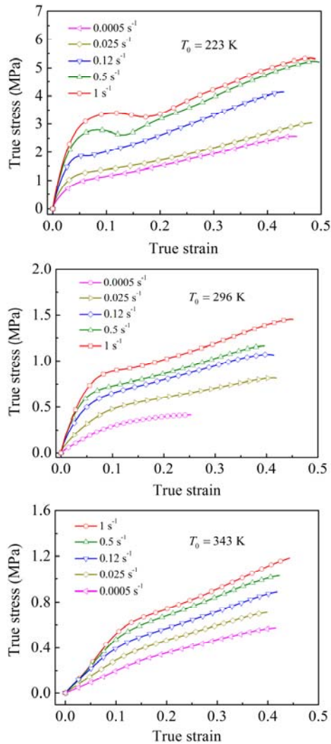
Fig. 5 Stress vs. strain curves at various temperatures
