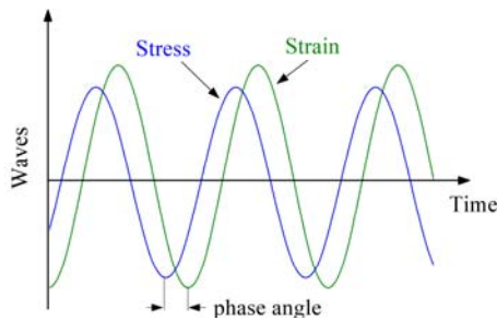
Fig. 8 The lag angle between stress and strain
