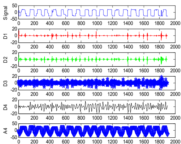
Fig. 1 Healthy VOG signal and wavelet coefficients
