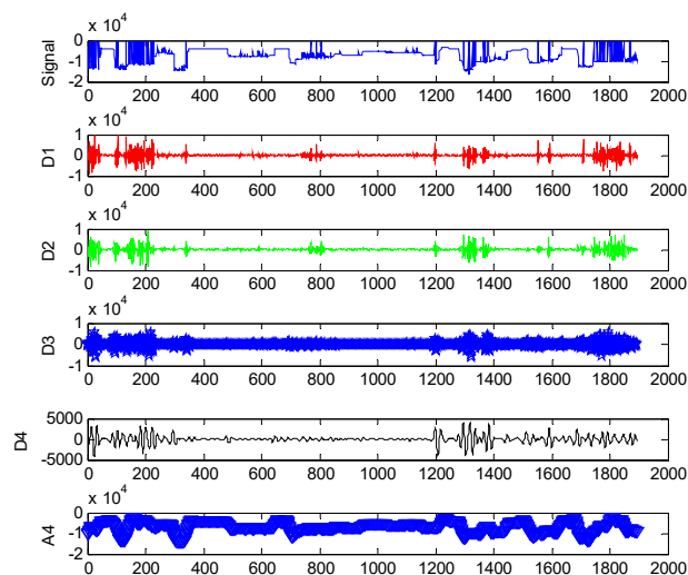
Fig. 3 PDR VOG signal and wavelet coefficients
