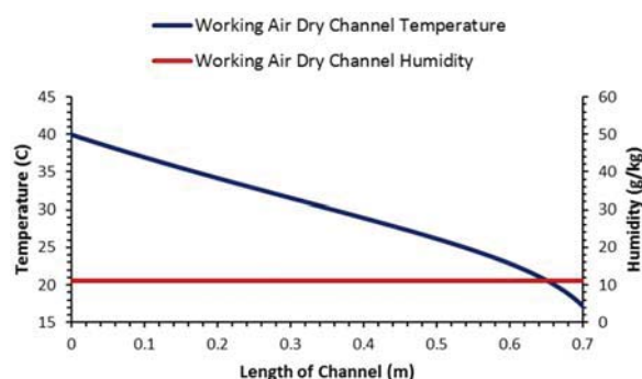
Fig. 7 Working Air-Dry Channel Temperature & Humidity Plot
