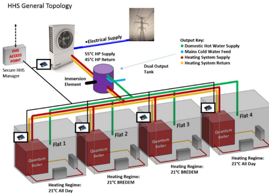
Fig. 9 Schematic of RISE Configuration for MDU
