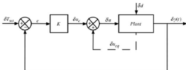
Fig. 3 RIDE/Inverse Dynamics control structure
