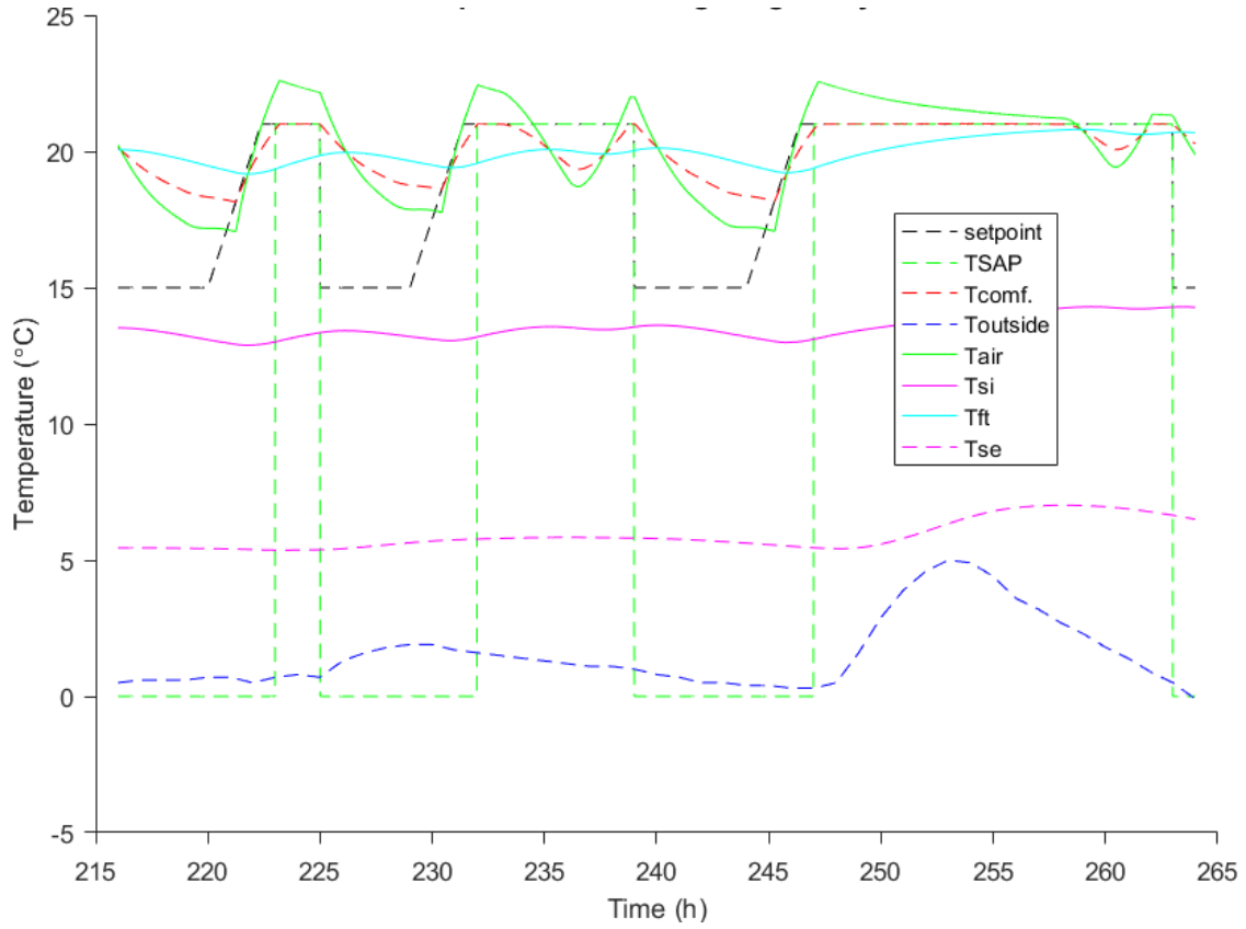
Fig. 6 Simulated result of RISE system performance
