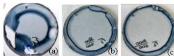
Fig. 2 Spin coating parameters optimization results for the deposition of a PEDOT layer with PEG 6 kDa 1.45 M/ml of Baytron C used in the oxidant solution. The spinning time has been kept constant (60 s) The used accelerations and speed are: a) 250 rpm/s, 500 rpm; b) 400 rpm/s, 800 rpm; c) 500 rpm/s, 1000 rpm
