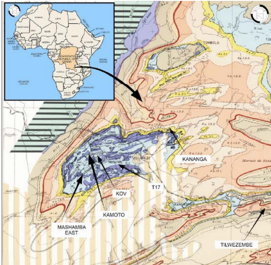
Fig. 3 (a) KOV geological settings (by SRK consulting)
