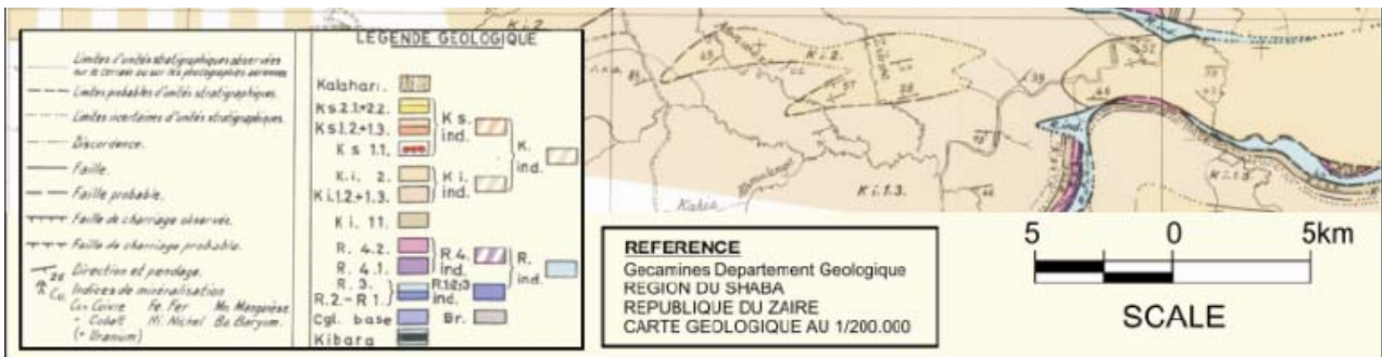
Fig. 3 (b) KOV geological settings (legend)
