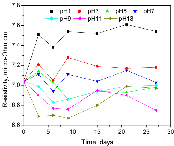
Fig. 4 The change of resistivity of Al-19Si automotive alloy as a function of immersion time at various pH environments
