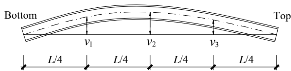
Fig. 4 Measurement of geometric imperfections
