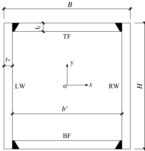
Fig. 1 Definition of symbols for a column section
