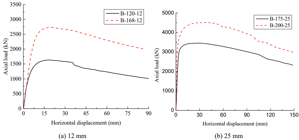
Fig. 6 Axial load-horizontal displacement curves of steel columns
