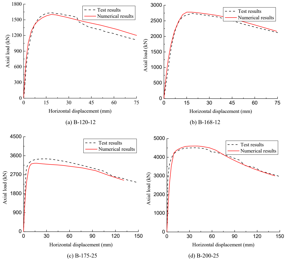
Fig. 8 Comparisons between experimental and numerical results
