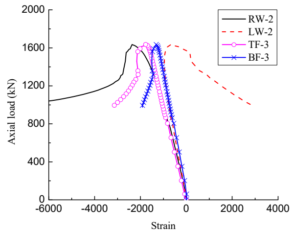
Fig. 5 Load-strain curves of steel column B-120-12
