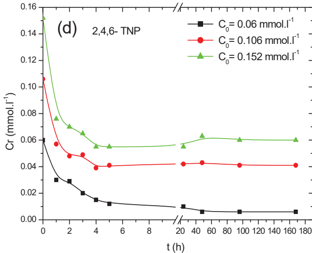
Fig. 3 Evolution of residual concentration ( c_r ) of the solution in the liquid phase of contact time ( t ) at natural pH
