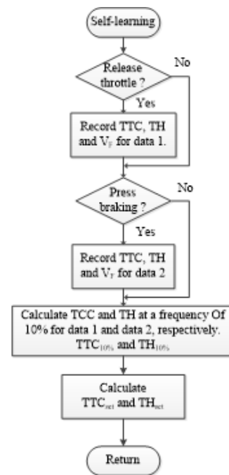
Fig. 4 A flowchart of the self-learning algorithm for the forward collision warning system
