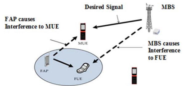
Fig. 3 Cross tier inter-cellular interference
