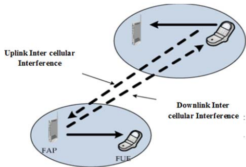
Fig. 2 Co tier inter-cellular interference
