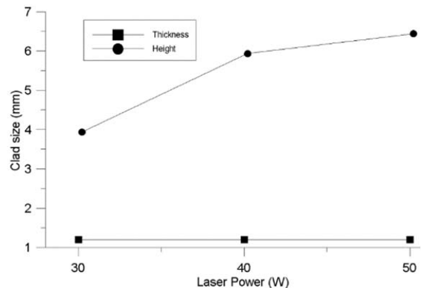
Fig. 11 Relationship between the clad height and laser power
