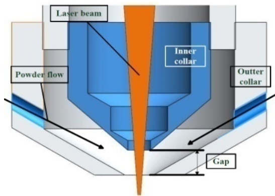
Fig. 3 Cladding nozzle drawing
