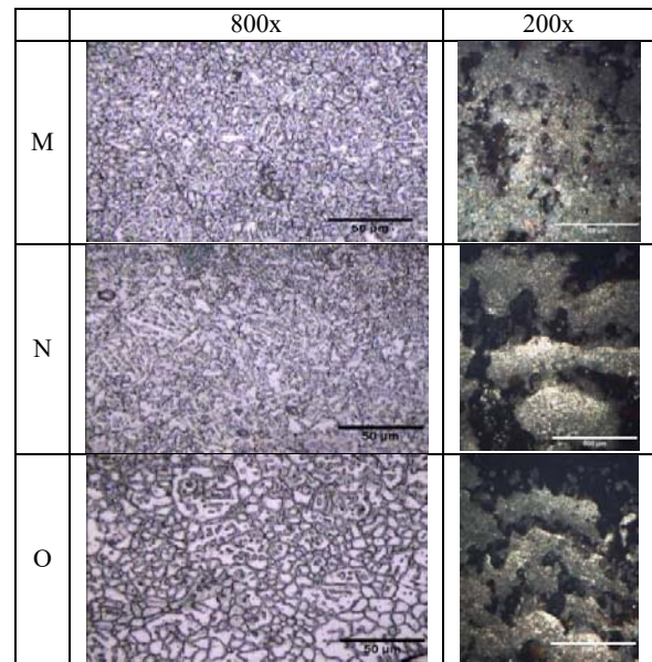
Fig. 15 Microstructure at different layer
