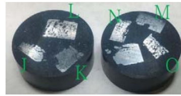
Fig. 14 Metallographic specimen
